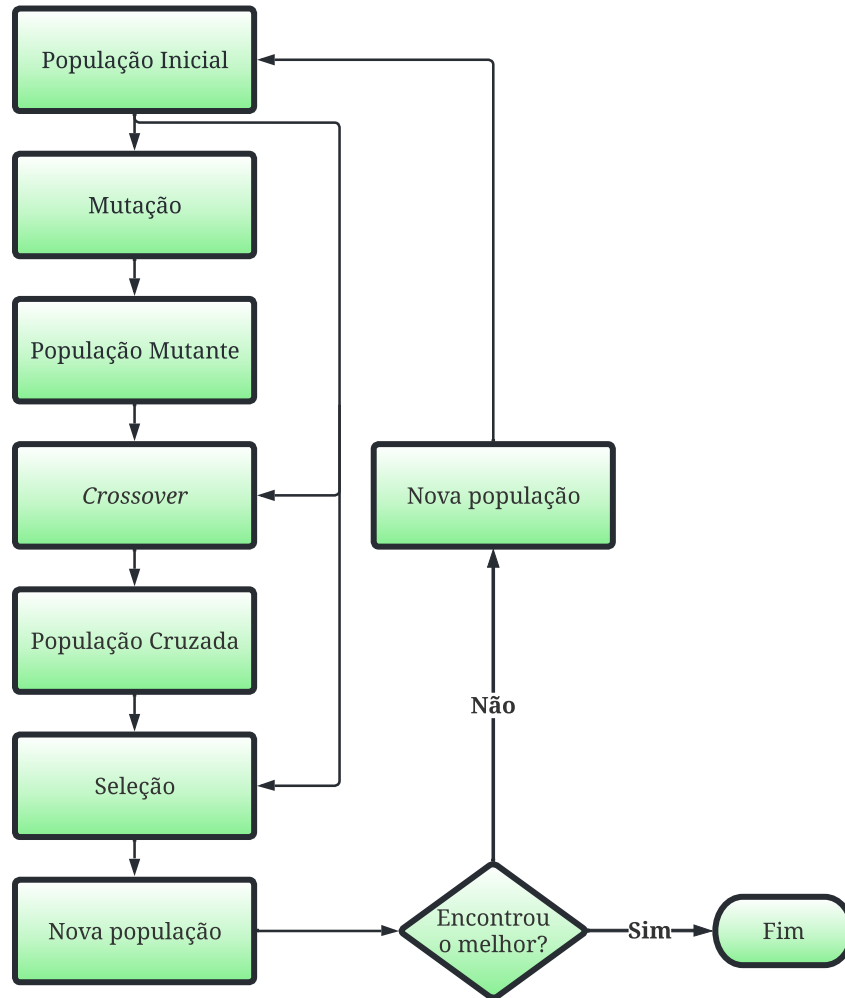
Figura 10 – Fluxograma do algoritmo Differential Evolution .
